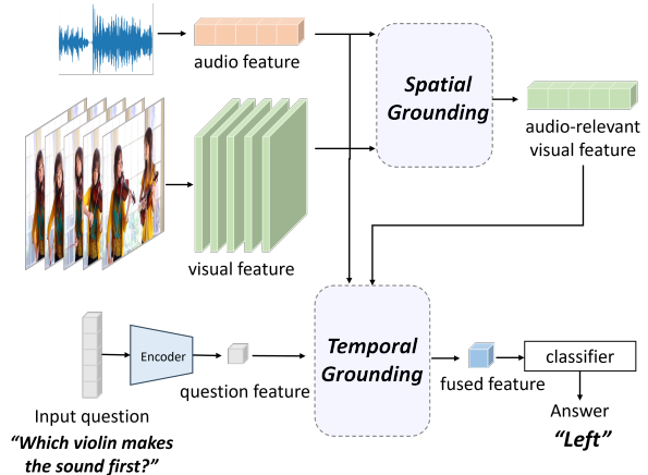
Figure 1: Our AVQA framework.
