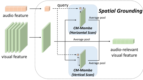
Figure 3: Audio-Guided Spatial Grounding.
