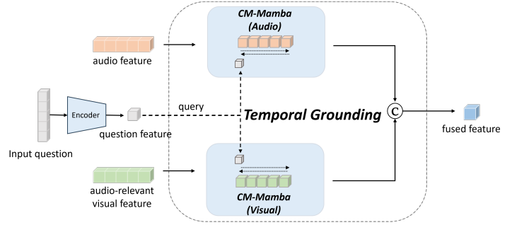
Figure 4: Question-Guided Cross-Modal Temporal Grounding.
