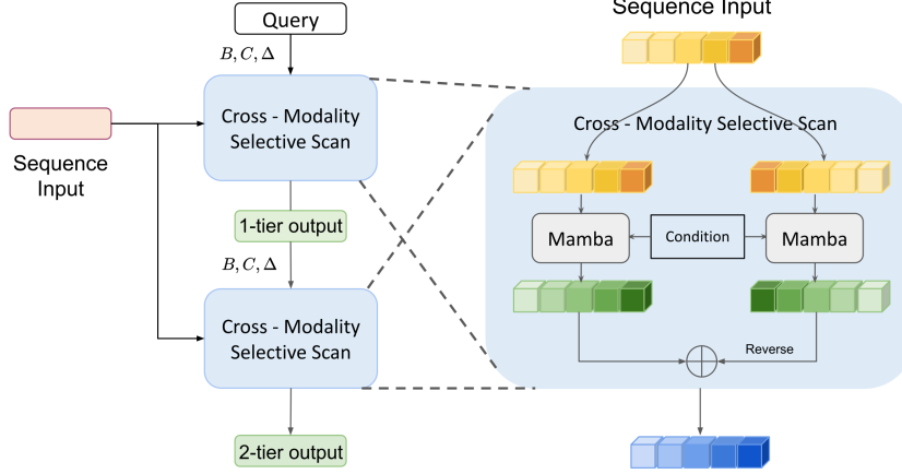
Figure 2: Our proposed CM-Mamba. Within each Cross-Modality Selective Scan block, bidirectional Mamba parameters are dynamically generated from the conditional information. The query serves as the condition for the first tier, while the output from the first tier serves as the condition for the second tier.
